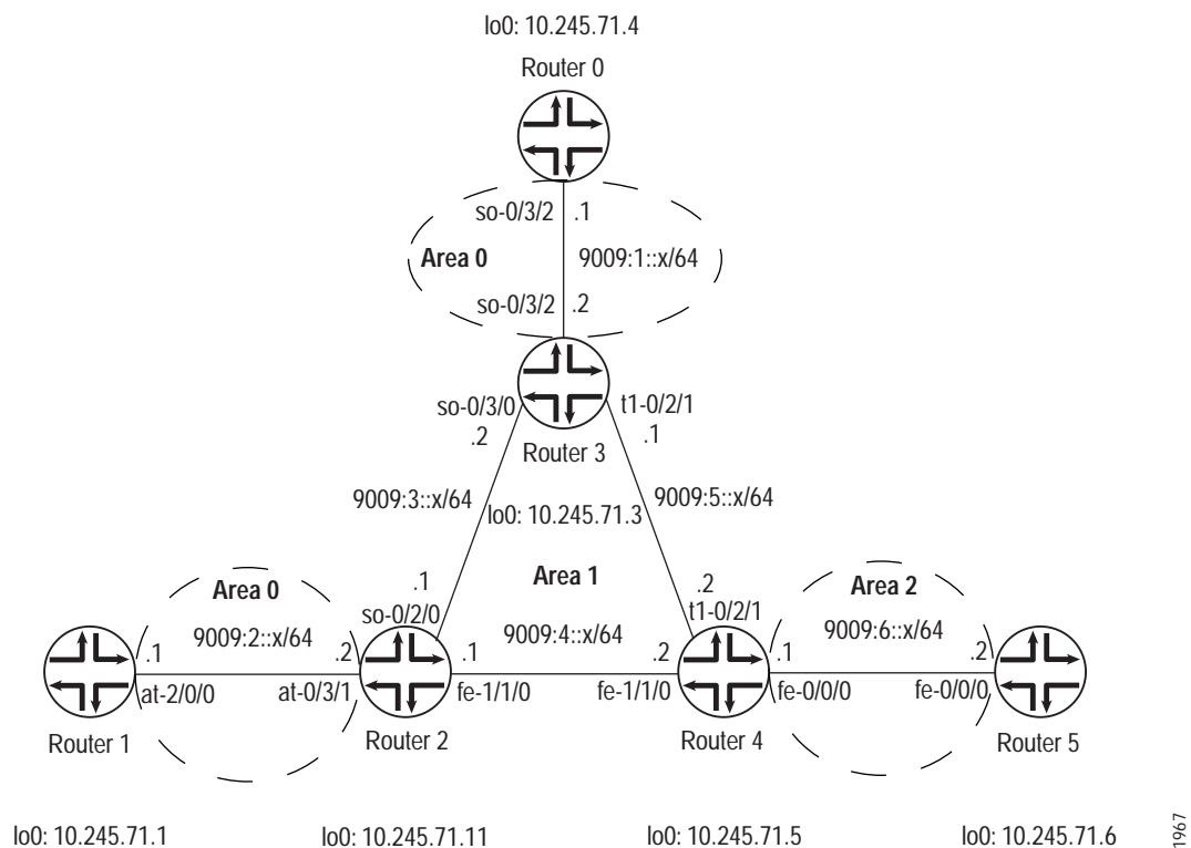
Figure 34: OSPFv3 for IPv6 Topology Diagram
