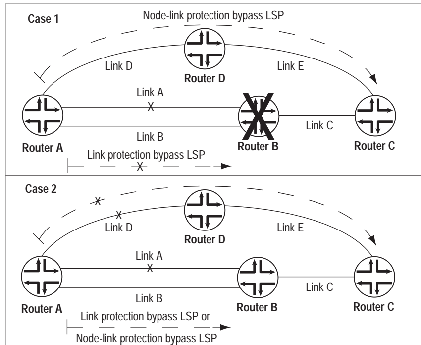
Figure 24: Link Protection and Node-Link Protection Comparison
