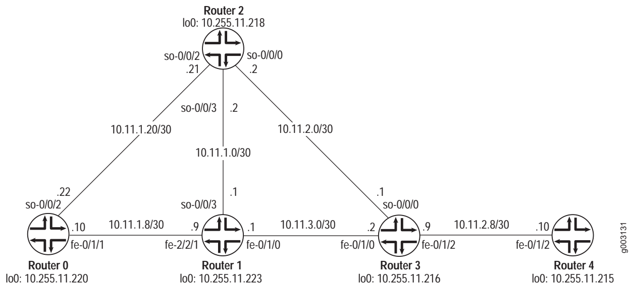
Figure 26: Node-Link Protection Topology Diagram
