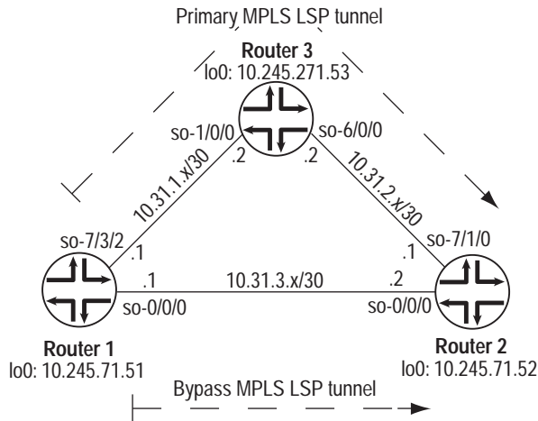
Figure 25: MPLS LSP Link Protection Topology Diagram
