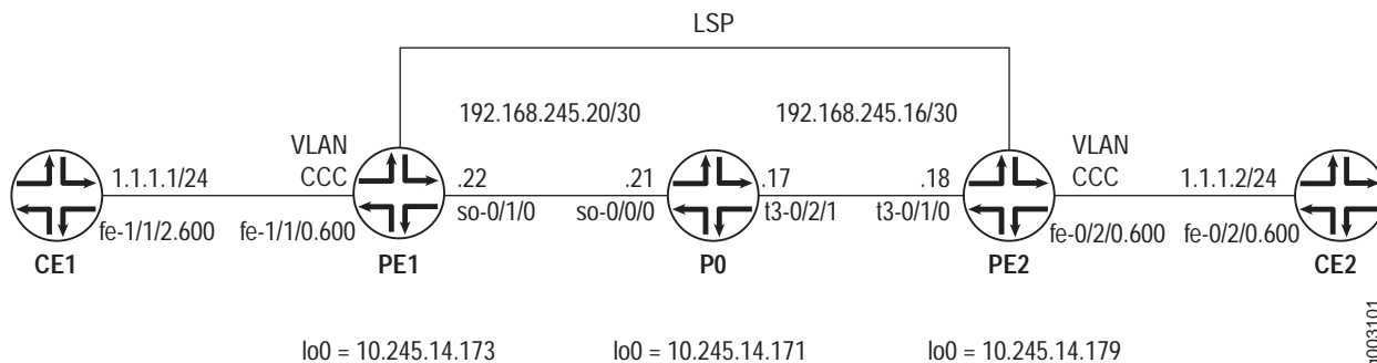
Figure 60: Ethernet-Based Layer 2 Circuit Topology Diagram
