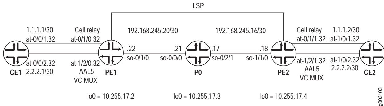
Figure 62: ATM2 IQ-Based Layer 2 Circuit Topology Diagram
