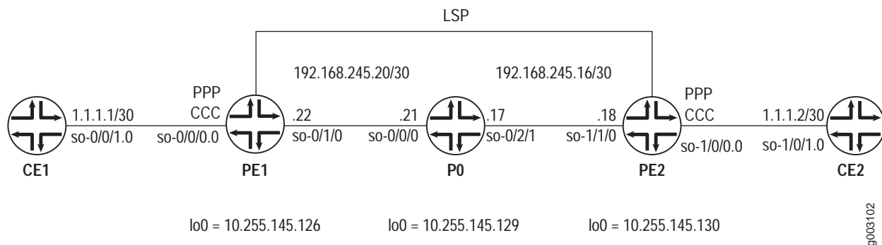
Figure 61: SONET/SDH-Based Layer 2 Circuit Topology Diagram
