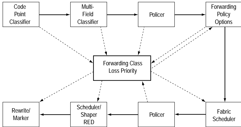
Figure 9: Packet Flow Through CoS-Configurable Components
