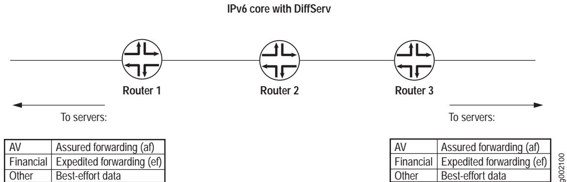
Figure 10: Basic IPv6 DiffServ Topology
