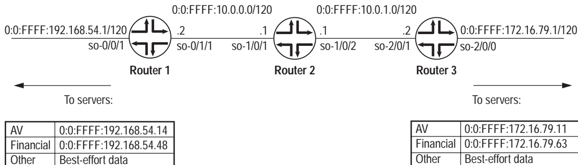
Figure 11: IPv6 DiffServ Configuration
