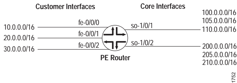
Figure 27: DCU/SCU Concept
