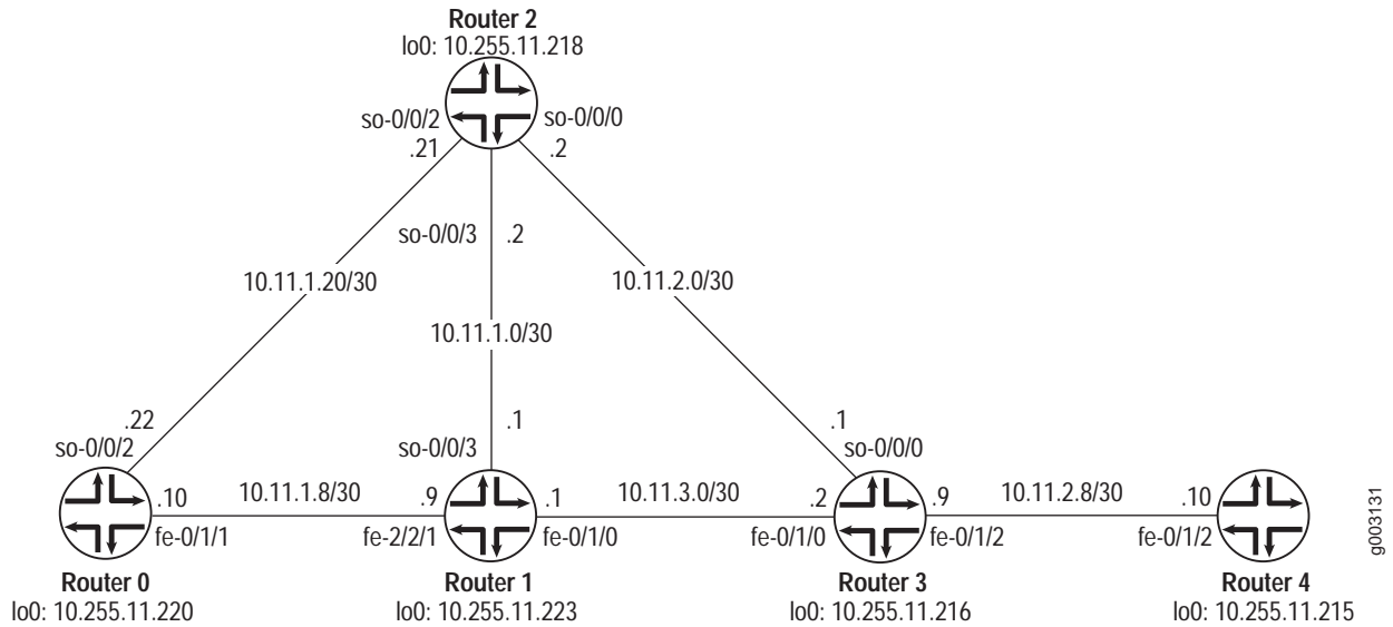
Figure 39: Node-Link Protection Topology Diagram
