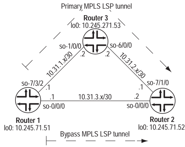
Figure 38: MPLS LSP Link Protection Topology Diagram
