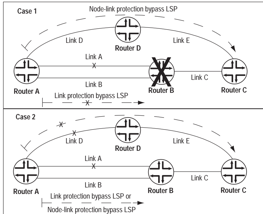
Figure 37: Link Protection and Node-Link Protection Comparison
