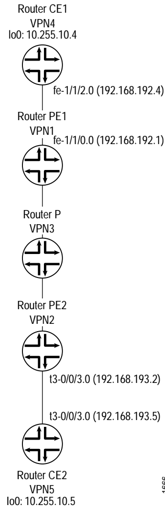
Figure 19: Layer 3 VPN Topology for ping and traceroute Examples
