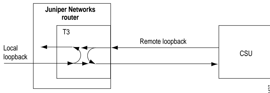
Figure 35: Remote and Local T3 Loopback
