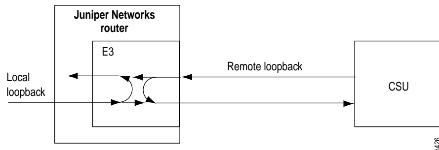
Figure 25: Remote and Local E3 Loopback
