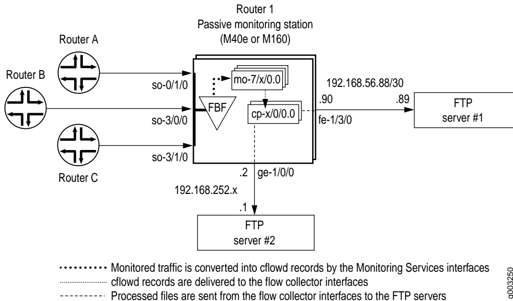
Figure 6: Flow Collector Interface Topology Diagram
