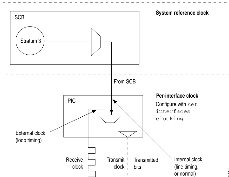
Figure 2: Clock Sources
