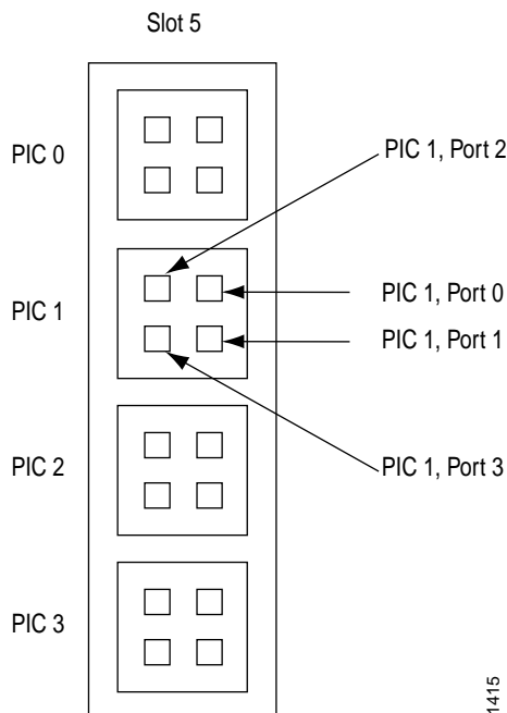
Figure 1: Interface Slot, PIC, and Port Locations
