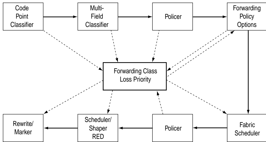
Figure 32: Packet Flow Through CoS Configurable Components
