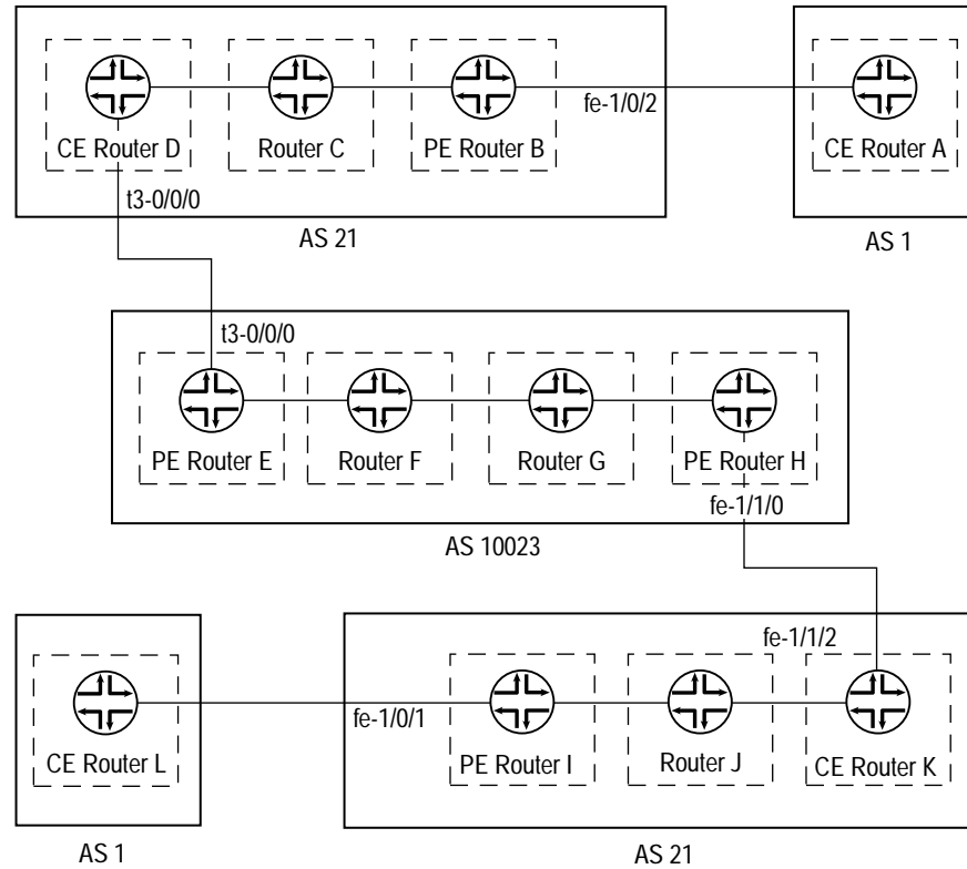
Figure 28: Carrier-of-Carriers Example
