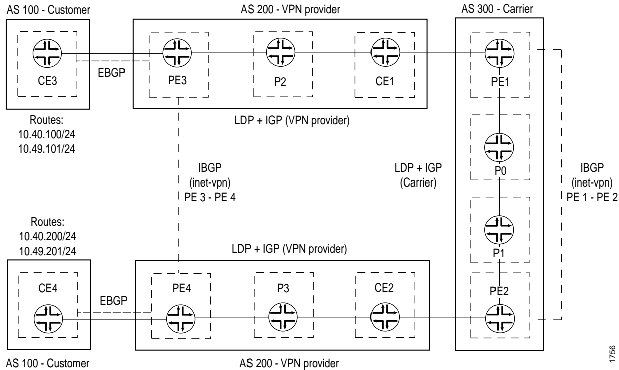
Figure 29: Multiple-Instance LDP Topology Diagram
