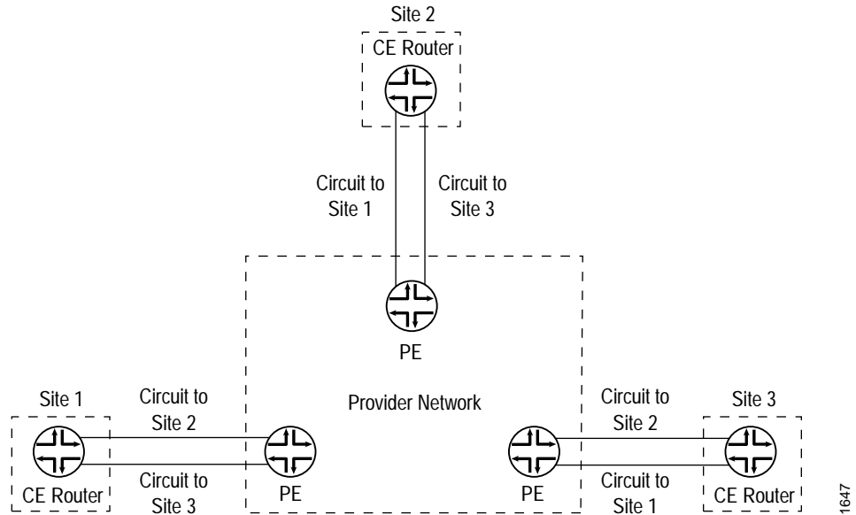
Figure 3: Layer 2 VPN Connecting CE Routers
