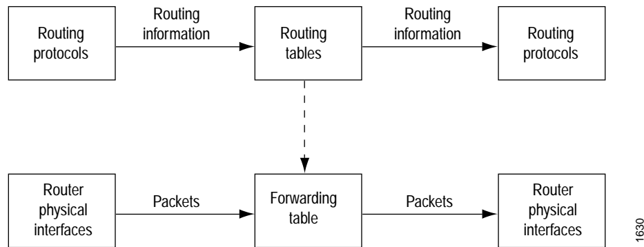
Figure 1: Flows of Routing Information and Packets
