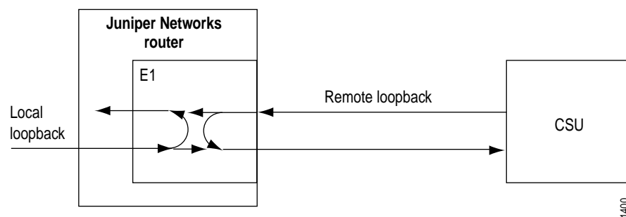
Figure 18: Remote and Local E1 Loopback
