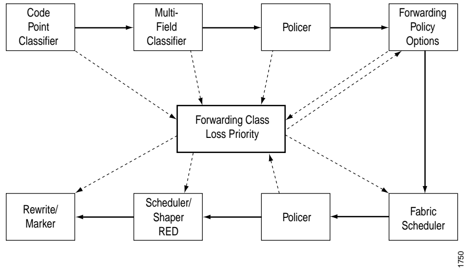
Figure 30: Packet Flow Through CoS Configurable Components
