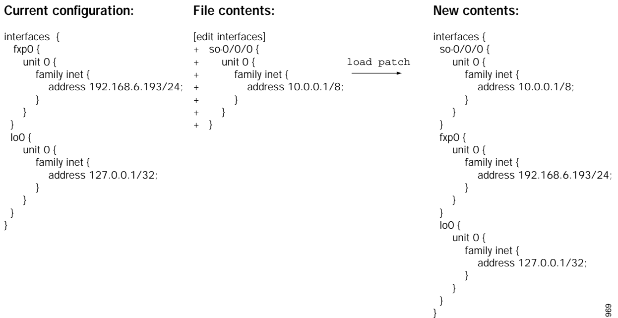
Figure 9: Example 4: Load Configuration from a File
