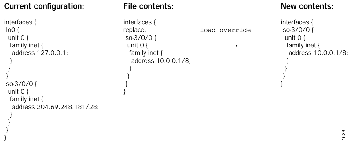
Figure 7: Example 2: Load a Configuration from a File
