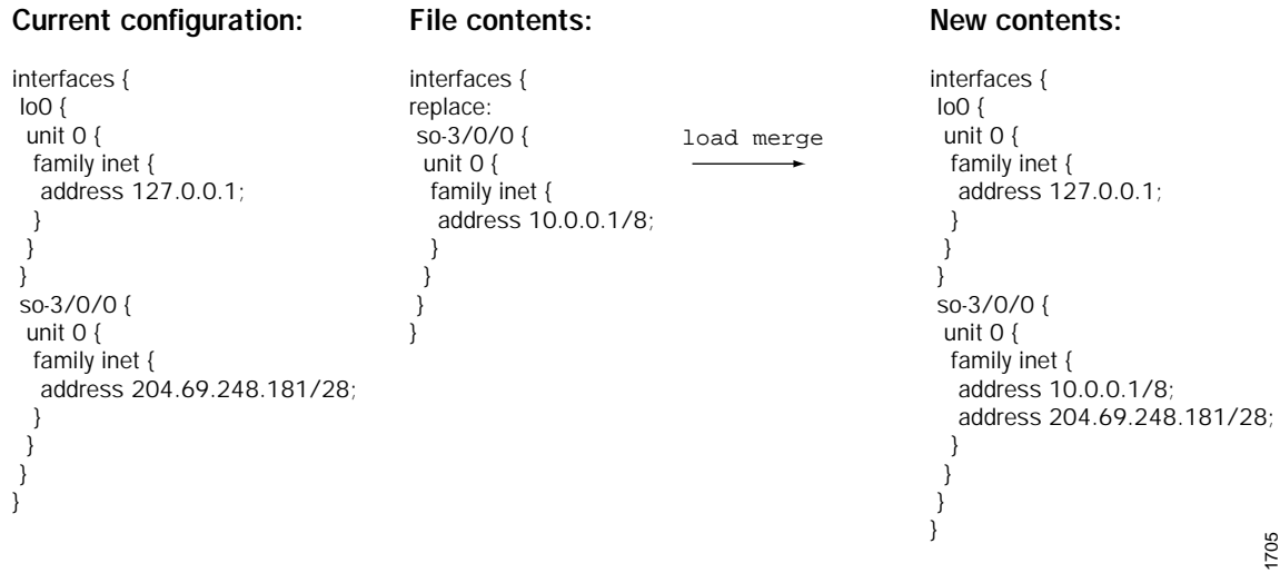
Figure 9: Example 4: Load Configuration from a File
