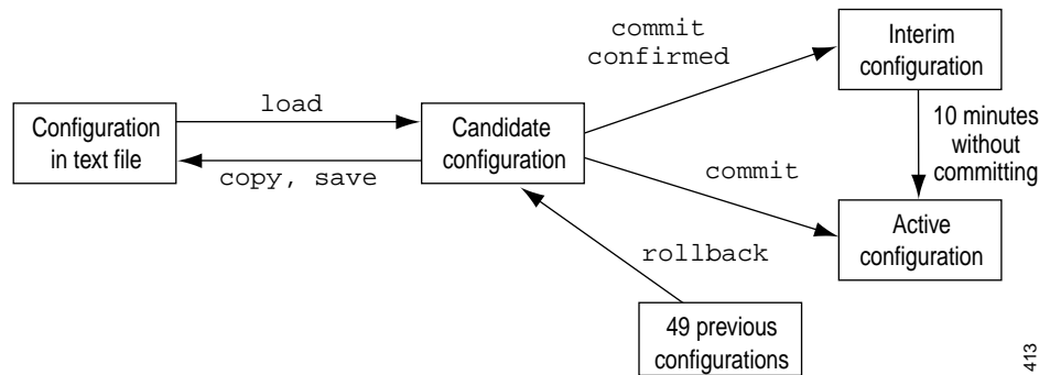
Figure 4: Commands for Storing and Modifying the Router Configuration
