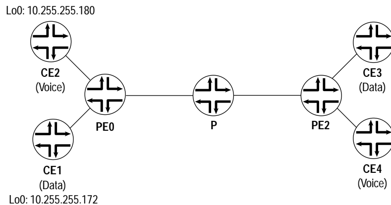
Figure 44: Non-Forwarding Instances Topology Diagram
