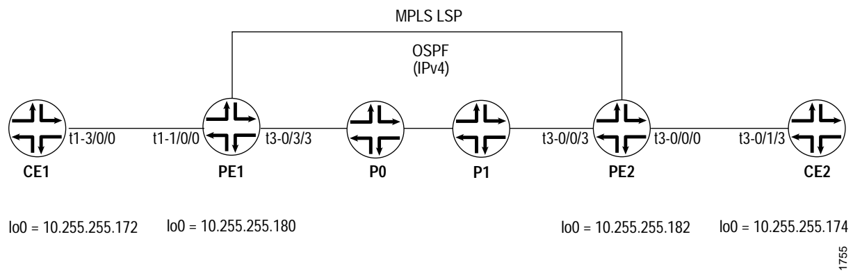
Figure 42: Overlapping VPNs Topology Diagram
