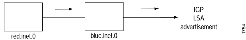
Figure 43: Non-Forwarding Instance Concept
