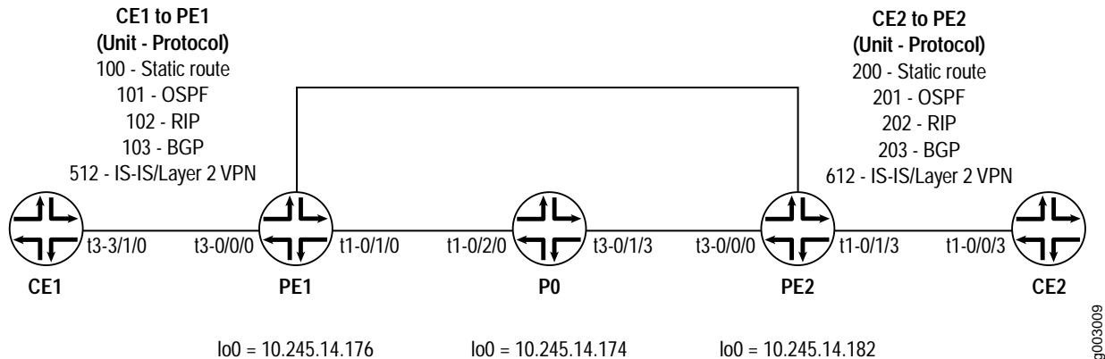
Figure 22: Layer 3 VPN Graceful Restart Topology Diagram
