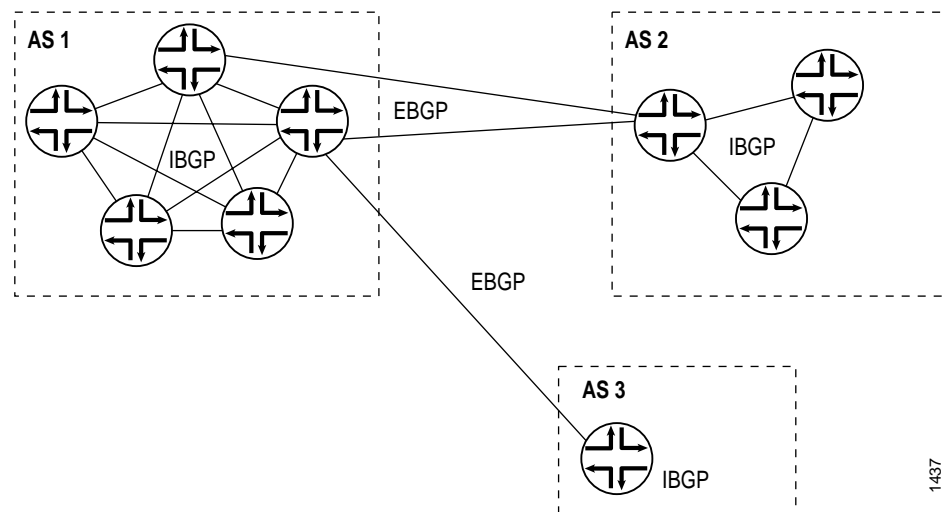
Figure 5: ASs, External BGP, and Internal BGP
