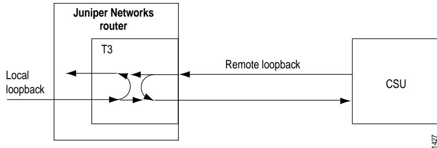
Figure 14: Remote and Local T3 Loopback
