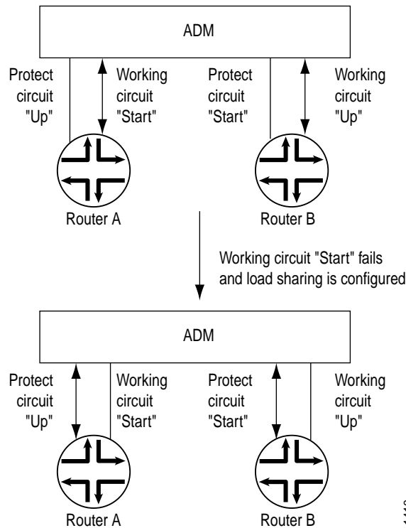
Figure 12: APS Load Sharing between Circuit Pairs
