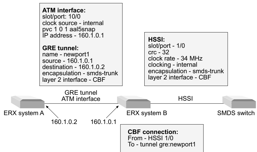
Figure 20-6 Sample SMDS configuration
