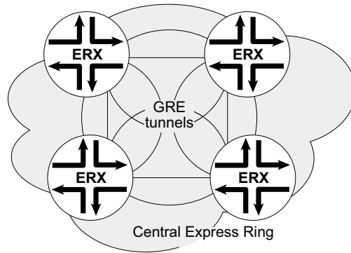
Figure 20-2 ERX system with GRE tunnels to offload the central express ring
