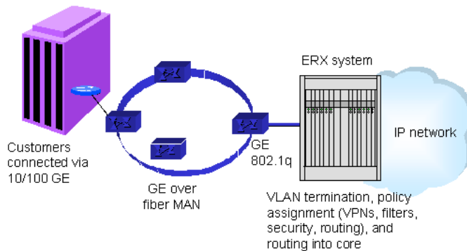
Figure 6-4 ERX system in a business Ethernet application
