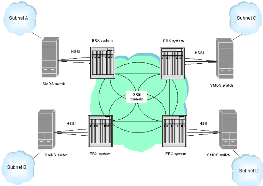
Figure 6-15 HSSI line modules in ERX systems provide connections to SMDS switches
