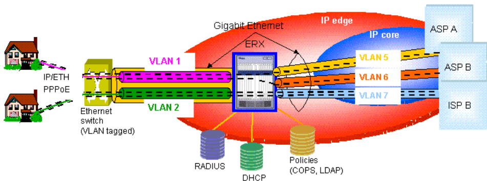
Figure 6-12 VLAN application with the ERX system
