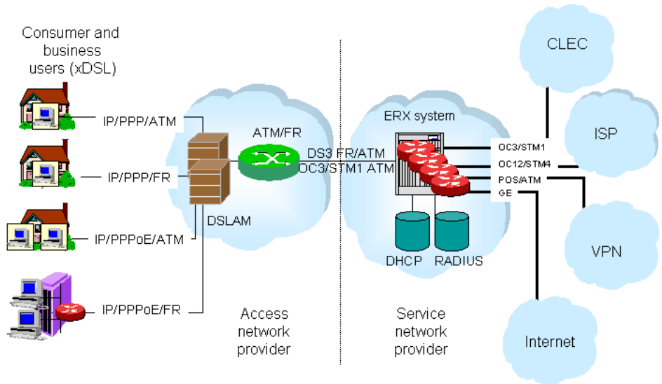
Figure 6-2 xDSL aggregation with the ERX system
