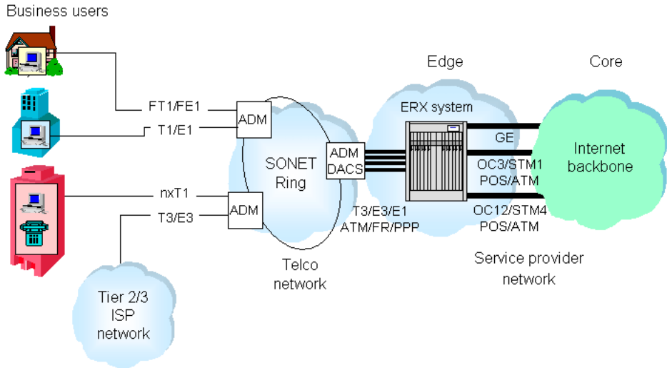
Figure 6-1 Private line aggregation application
