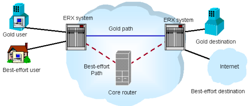
Figure 6-7 MPLS use for traffic engineering
