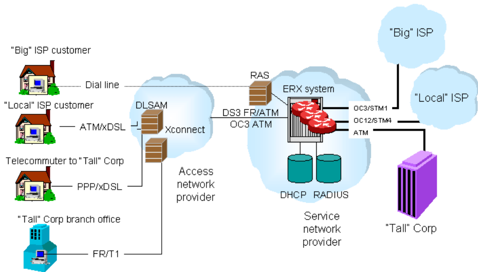
Figure 6-5 Delivery of VPNs over a shared IP infrastructure
