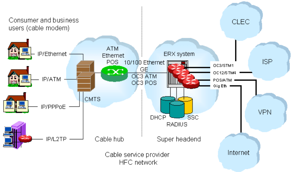
Figure 6-6 Cable subscriber management application
