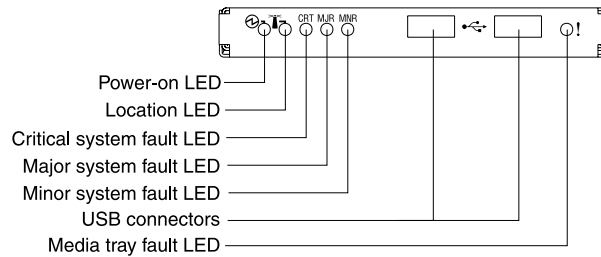
Figure 1: JCS1200 Media Tray Components
