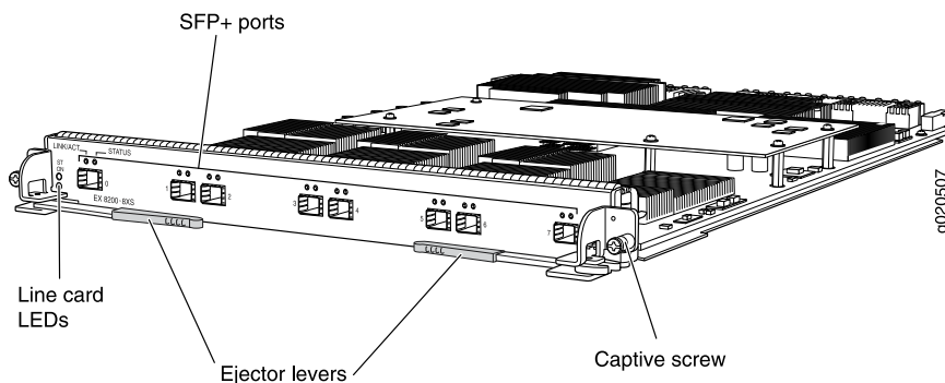
Figure 1: 8-port SFP+ Line Card
