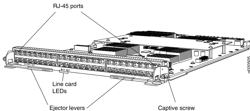
Figure 1: 48-port RJ-45 Line Card
