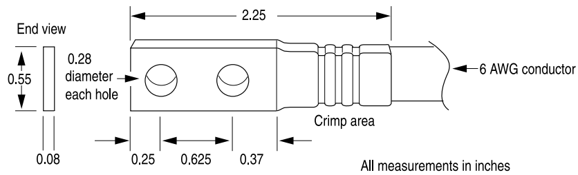
Figure 1: Grounding Cable Lug
