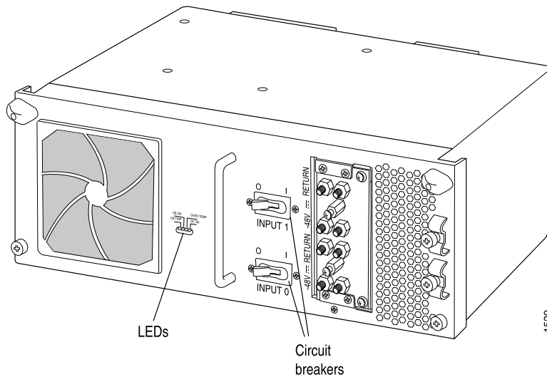
Figure 1: Power Supply
