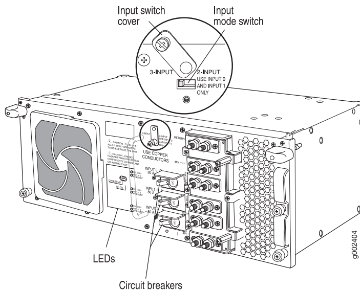
Figure 1: Three-Input 240-A Power Supply
