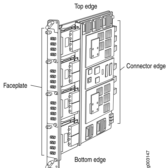
Figure 1: FPC Edges
