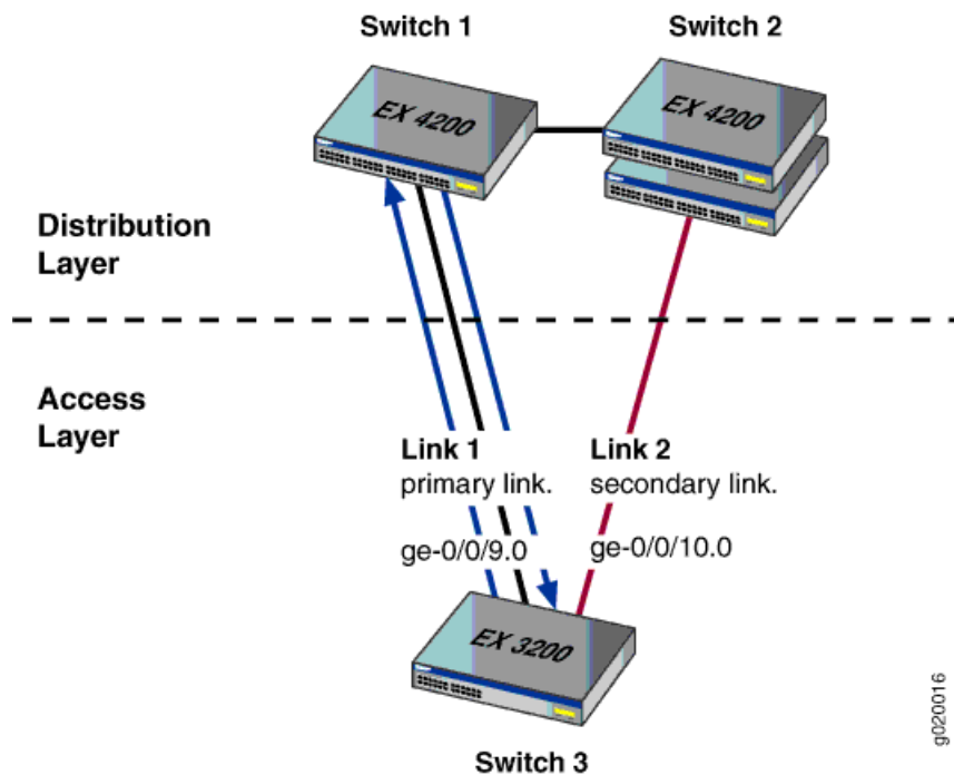
Figure 1: Topology for Configuring the Redundant Trunk Links
