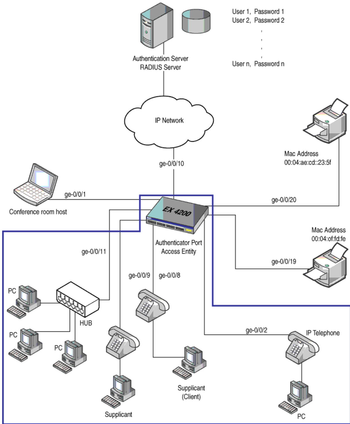
Figure 1: Topology for Configuring Supplicant Modes
