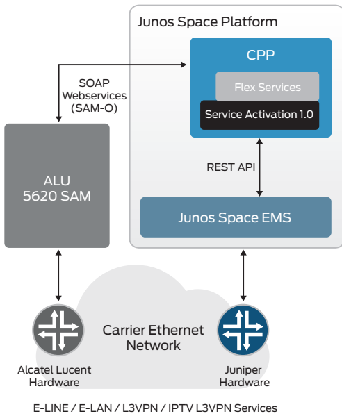
Figure 3. CPP integration with Alcatel-Lucent 5620 SAM
